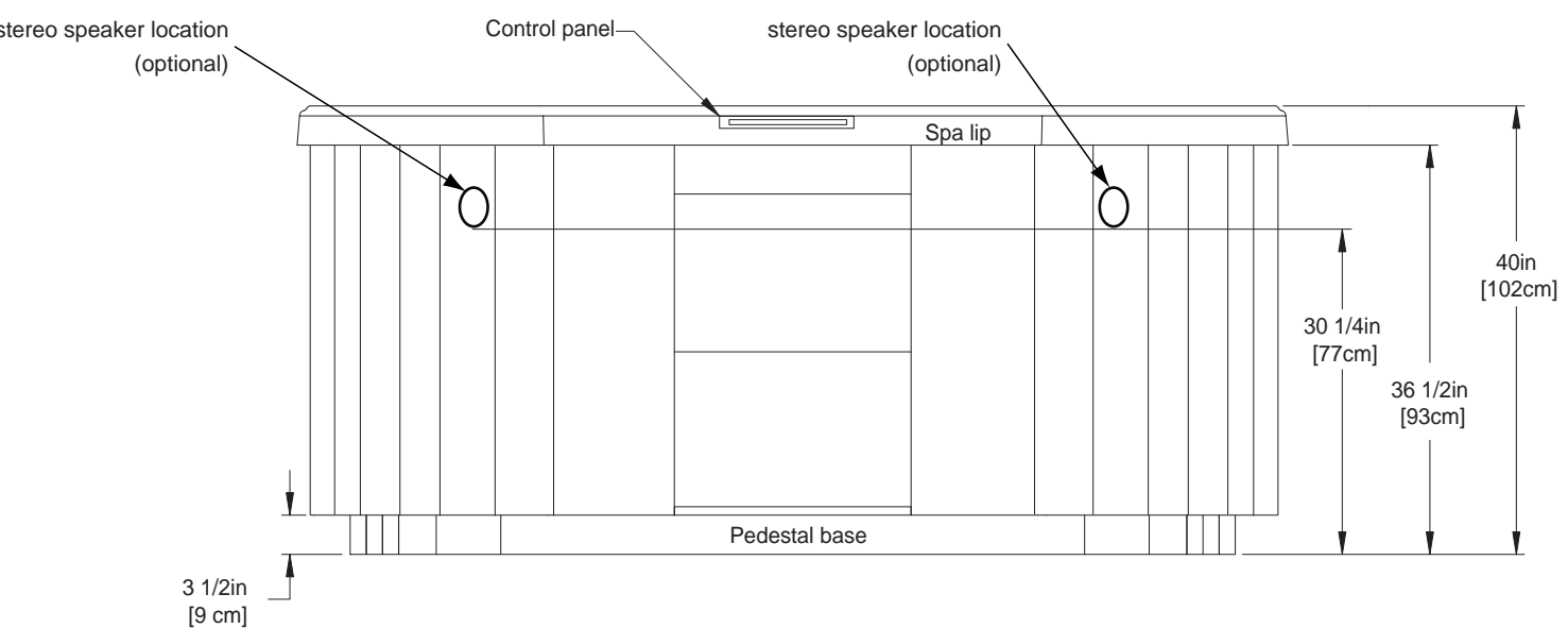
FRONT VIEW
